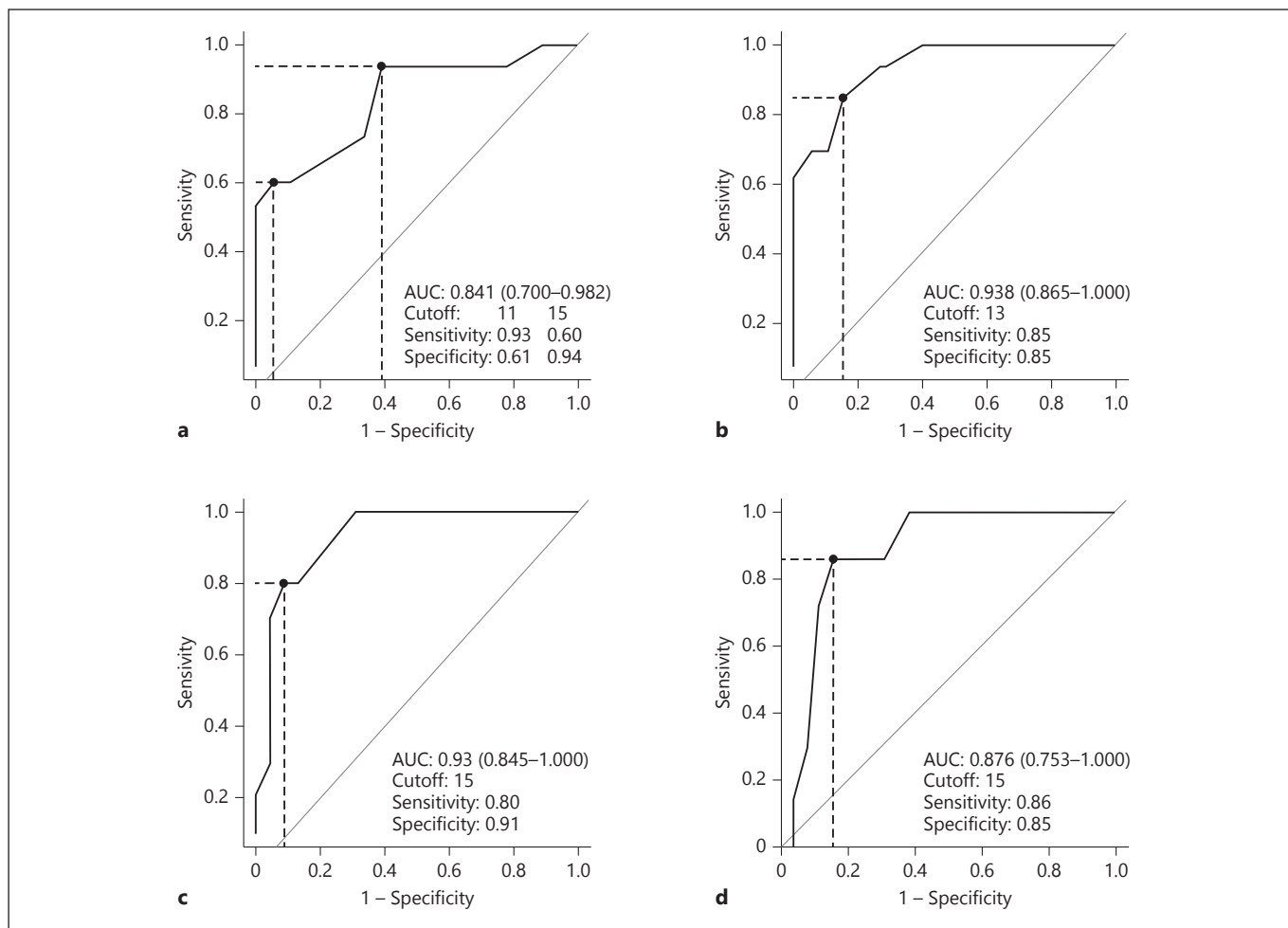
Fig. 1. ROC analysis for diagnostic accuracy of maximal Thompson-score for (a) surviving without cognitive impairment (alive and IQ \geq 85 ), (b) surviving without relevant neurological impairment, (c) surviving without development of epilepsy, (d) surviving
